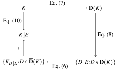
FIGURE 1. Commuting diagram for conditioning.
